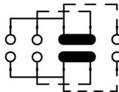
SCHEMATIC (SHORTING)
